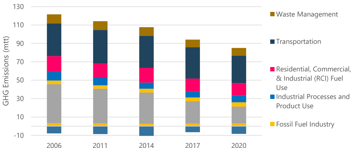
Figure 60. Total GHG Emissions in Maryland by Sector (2006-2020)
